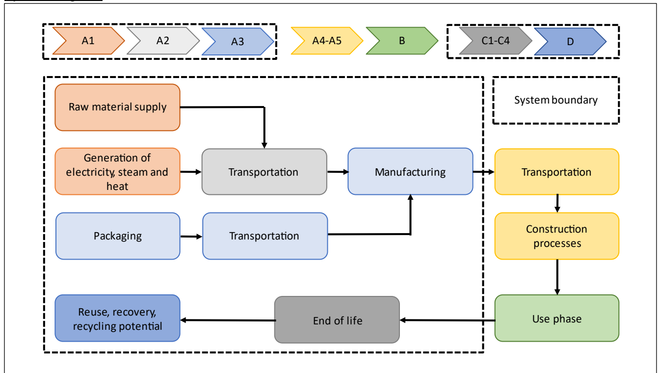
Figure 1 System boundary of the LCA study conducted on Fatra Garis - homogeneous floor covering
